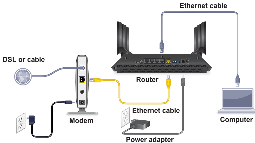
Figure 4. Router cabling
